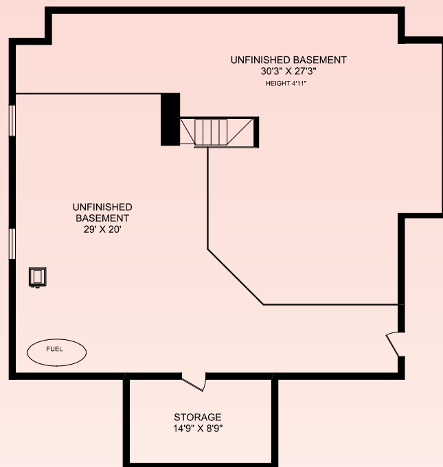
LOWER FLOOR
